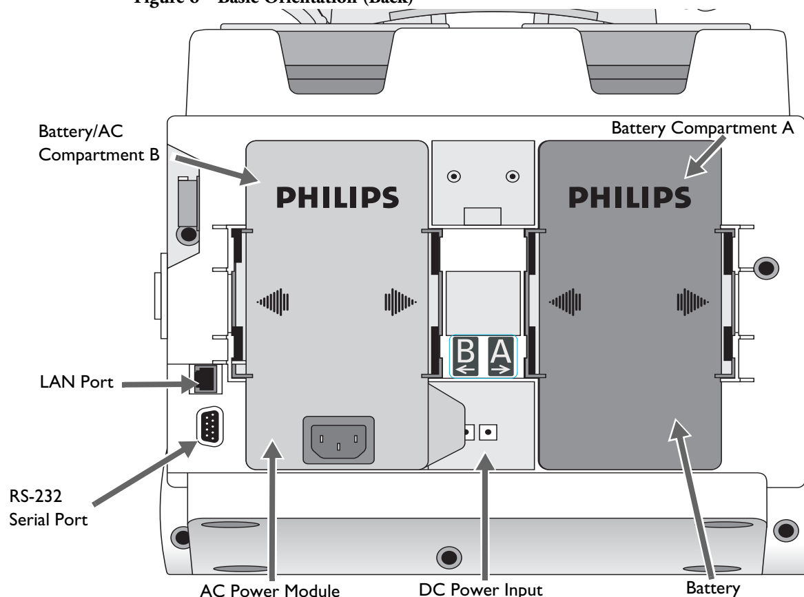
Figure 6 Basic Orientation (Back)
